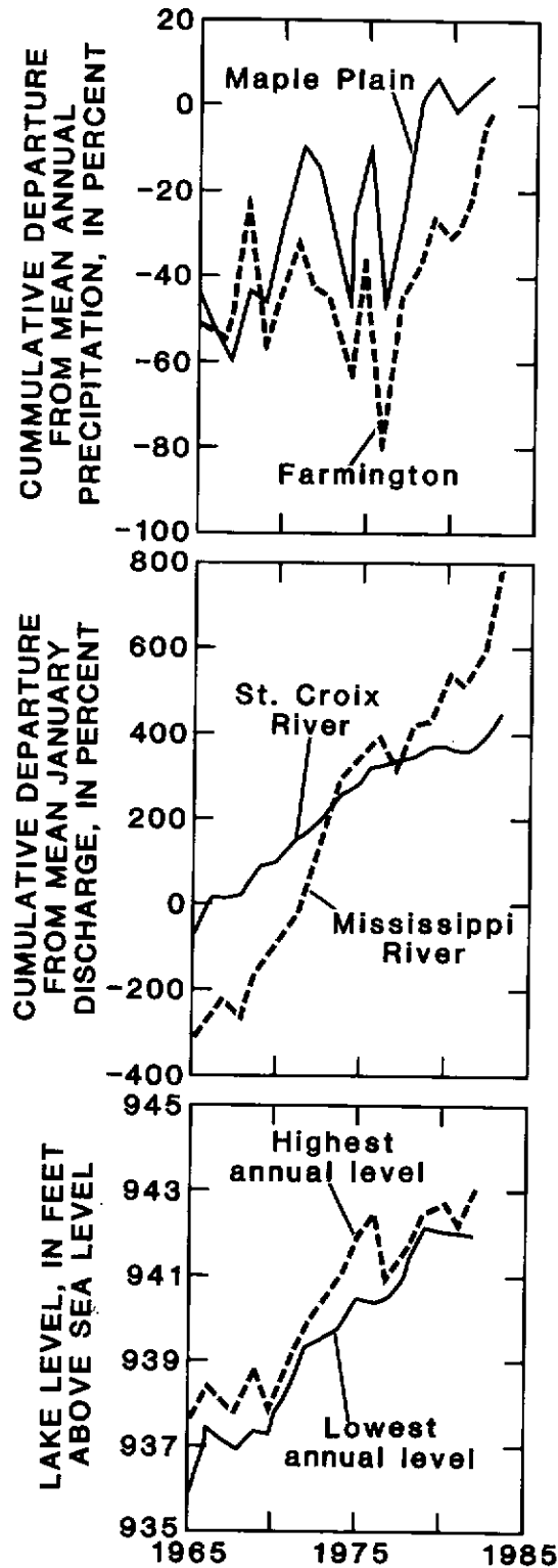
Figure 11.--Cumulative departure from mean annual precipitation at Maple Plain and Farmington, Minnesota; cumulative departure from mean January discharge of Mississippi River at St. Paul, Minnesota, and of St. Croix River at St. Croix Falls, Wisconsin; and annual high and low water levels of Big Marine Lake, 1965-82
